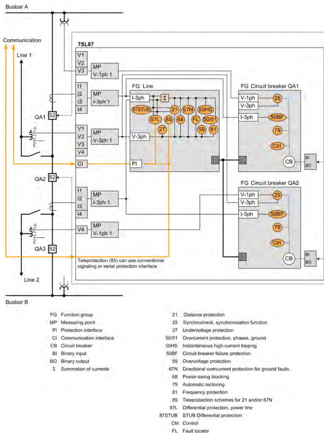
Figure 2.8/8 Application Example: Combined Line Differential and Distance Protection for Overhead Line with Breaker-and-a-Half Layout
