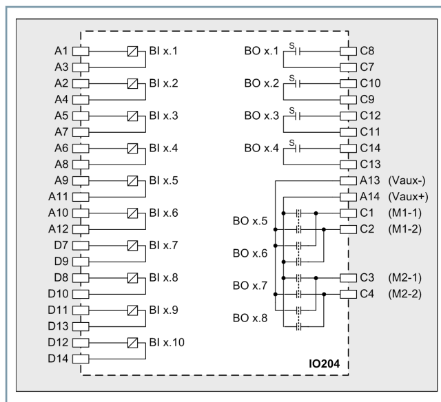
Figure 6.2/8 Connection Diagram IO204
