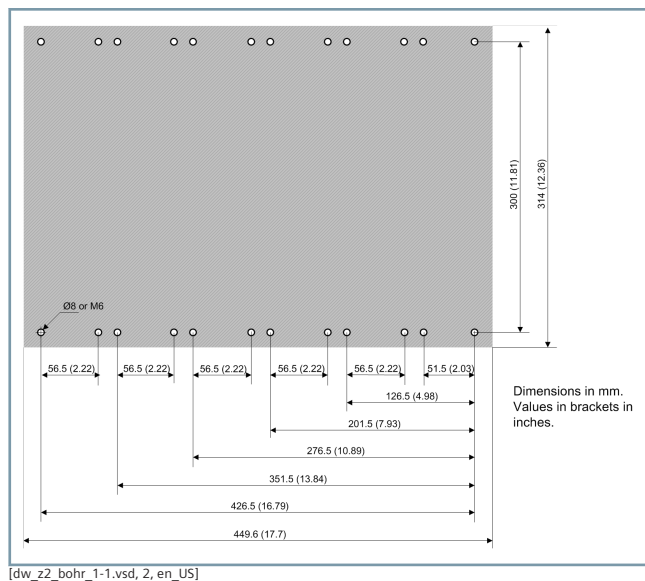
Figure 6.3/32 Drilling Pattern of a 1/1 Surface-Mounted Device – 2nd Device Row
