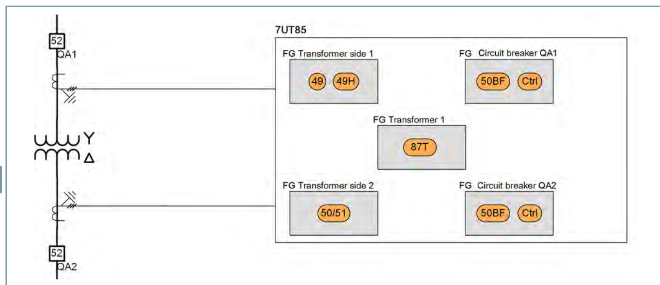
Figure 2.3/9 Two-Winding Transformer
