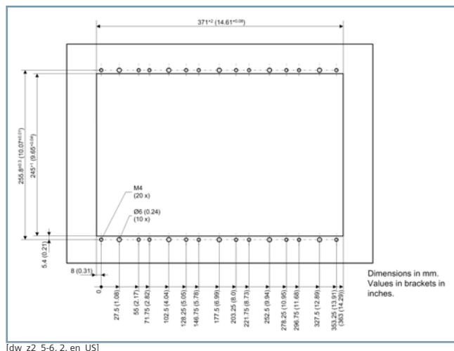
Figure 6.3/9 Cut-Out Widths and Drilling Pattern – 5/6 Device, 2nd Device Row
