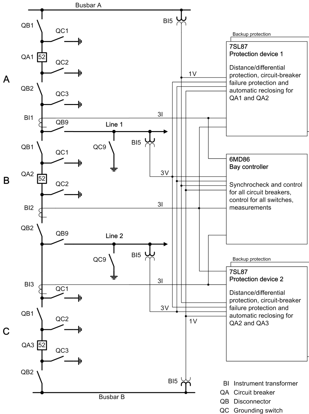
Figure 2.16/7 Breaker-and-a-Half Layout with a Bay Controller and 2 Line Protection Devices (Overview)
