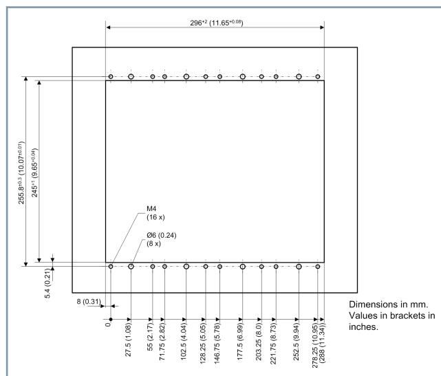
Figure 6.3/8 Cut-Out Widths and Drilling Pattern – 2/3 Device, 2nd Device Row
