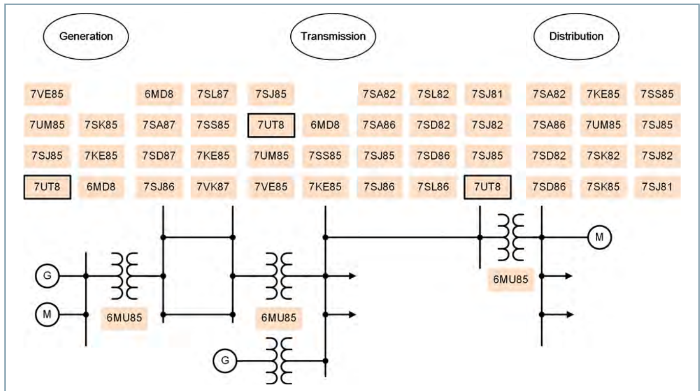
Figure 2.11/1 Fields of Application of the SIPROTEC 5 Devices
