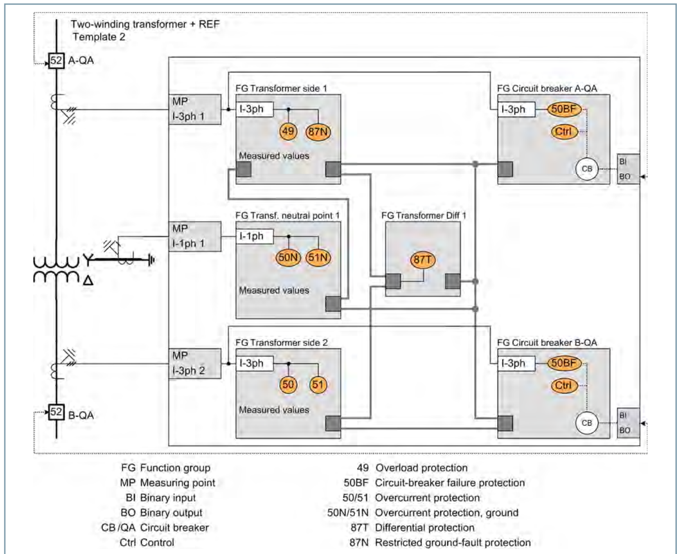
Figure 3.1/2 Transformer Protection
