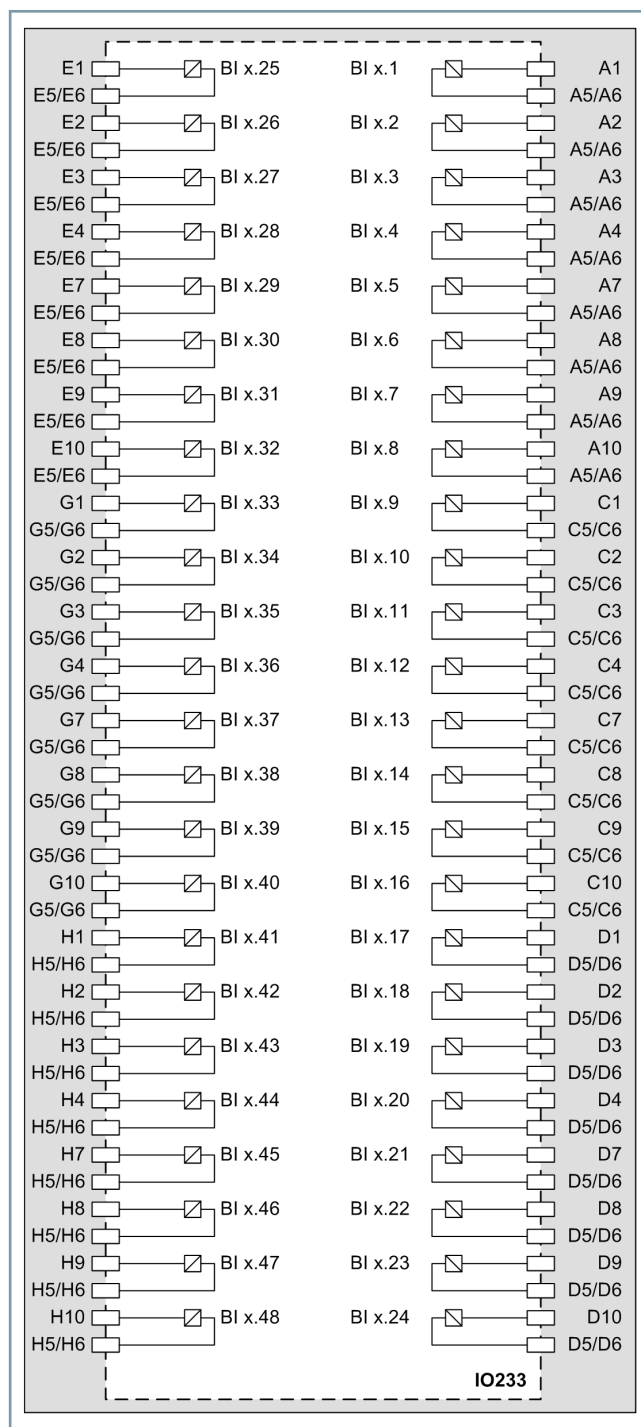
Figure 6.2/21 Connection Diagram IO233
