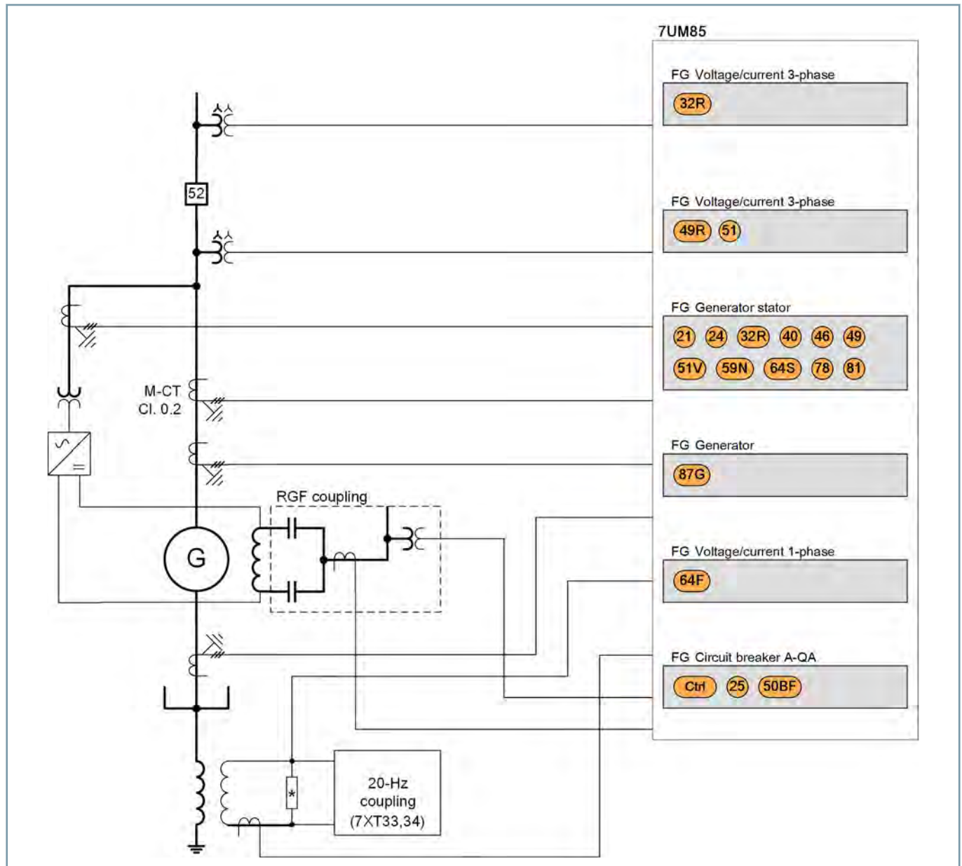
Figure 2.3/20 Protection of a High-Power Generator
