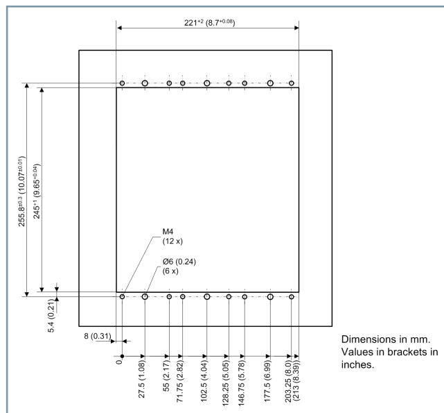
Figure 6.3/7 Cut-Out Widths and Drilling Pattern – 1/2 Device, 2nd Device Row
