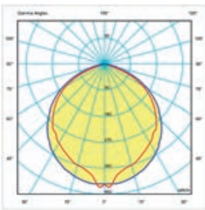
20 - Extra wide beam - 24W
