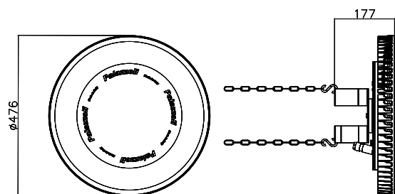
Adjustable double chain suspension
