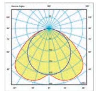
11 - T8 - 2 tubes - Symmetrical
