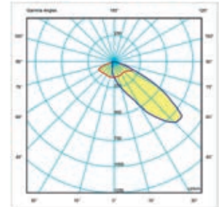
19 - Asymmetrical light distribution
