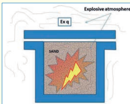
Picture 18: type of protection Ex q
