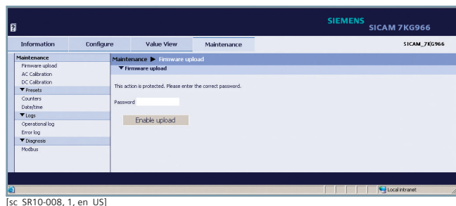
Figure 4.1/7 "Maintenance" Tab
