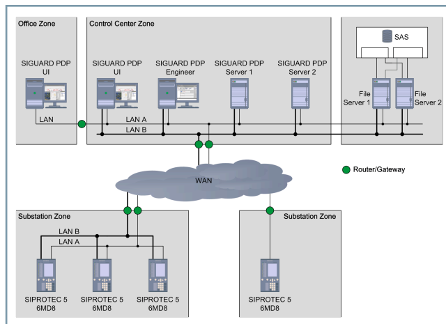
Figure 6.3/14 Redundant Configuration of the SIGUARD PDP Servers
