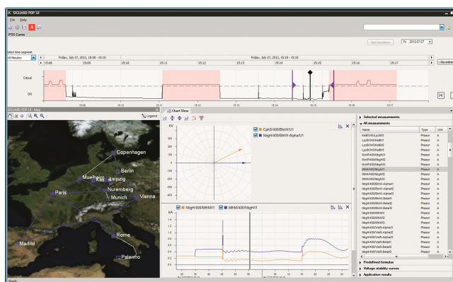
Figure 6.3/15 SIGUARD PDP User Interface (Example 1, Offline)
