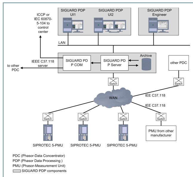
Figure 6.3/13 Structure of the SIGUARD Phasor Data Processing System
