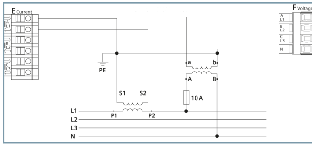
Figure 3.1/13 Connection Example 3-Wire Network, 1 Voltage and 1 Current Transformer, Any Load
