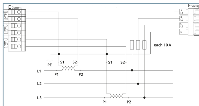
Figure 3.1/10 Connection Example 3-Wire Network, No Voltage Transformer and 2 Current Transformers, Any Load
