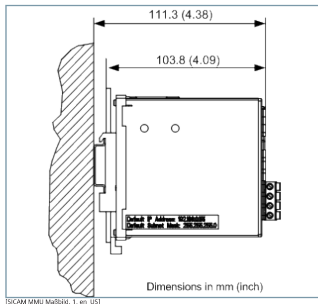
Figure 3.2/14 Dimensional Drawing of the SICAM MMU
