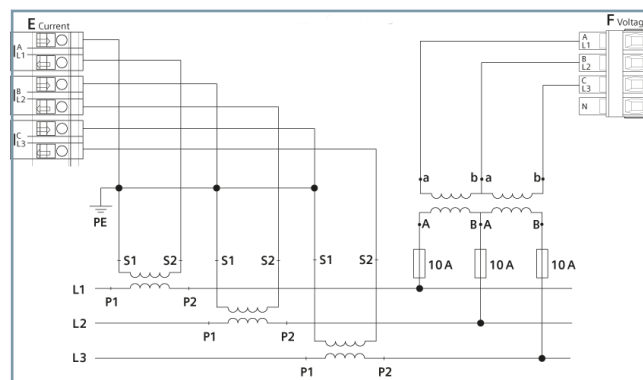
Figure 2.4/12 Connection Example 3-Wire Network, 2 Voltage and 3 Current Transformers, Any Load
