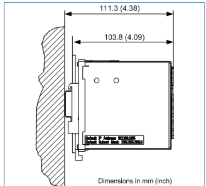
Figure 4.1/15 SICAM T Dimensions
