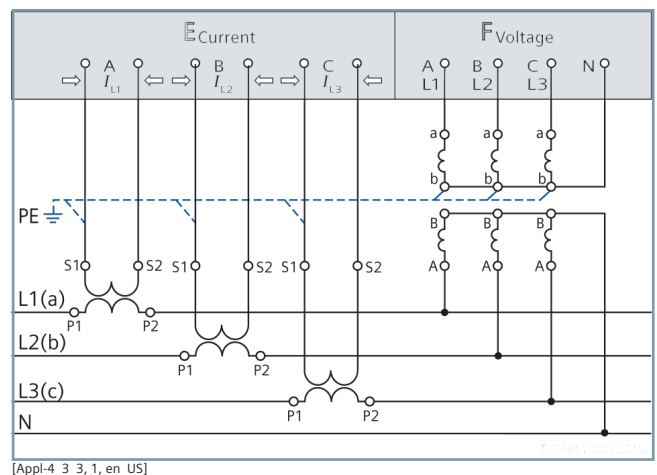
Figure 4.1/14 4-Wire Network, 3 Voltage and 3 Current Transformers, Any Load
