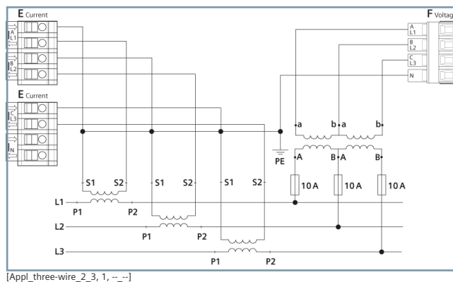
Figure 2.3/12 Connection Example 3-Wire Network, 2 Voltage Transformers and 3 Current Transformers, Any Load
