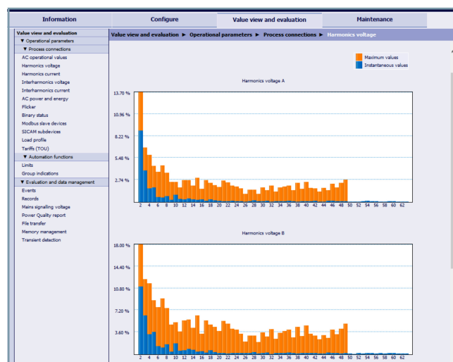
Figure 2.4/4 Graphical Representation of the Harmonics
