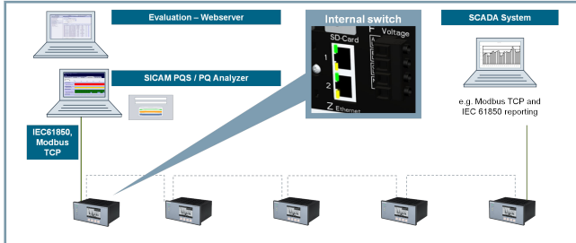
Figure 2.2/6 Example: Parallel Power-Quality Evaluation and Operating-Value Processing
