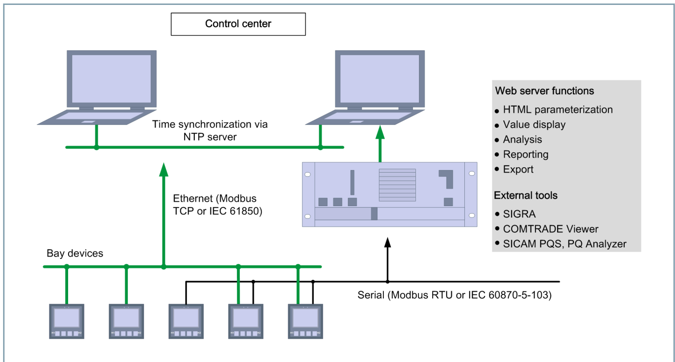
Figure 2.4/2 Application Example with SICAM P855
